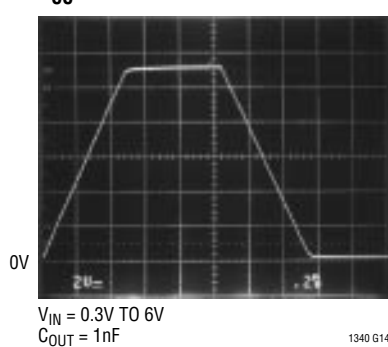
Rail-to-Rail Step Response at VCC = 6V
