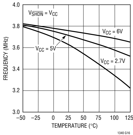
Charge Pump Frequency vs Temperature
